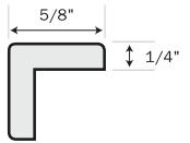
A105 Outside Corner
