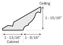
A100 Top Mount
