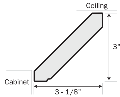
A140 Face Mount
