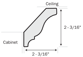
A101 Face Mount
