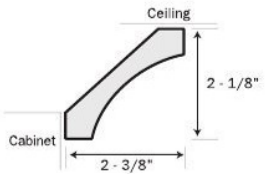
A114 Face Mount
