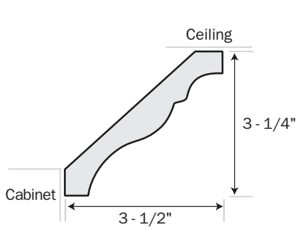
A115 - Face Mount
