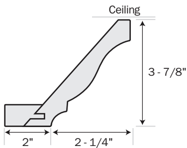
A131 - Top Mount
