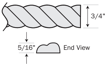
A108 - 3/4" Rope Molding
