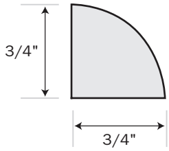
A104 - Shoe Molding
