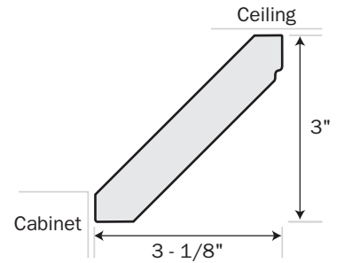
A140 - Face Mount
