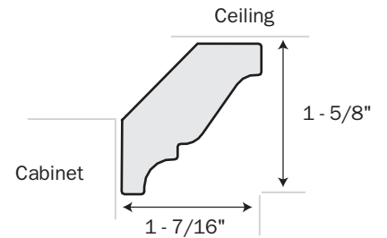
A102 - Face Mount
