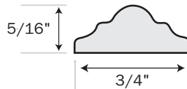
A111 - 3/4" Decorative Batten
