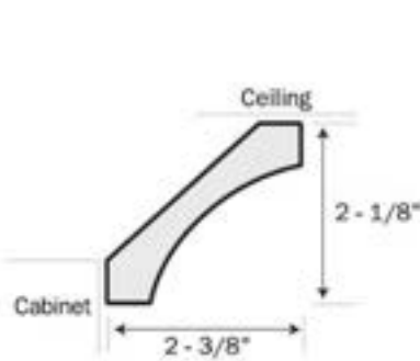
A114 Face Mount
