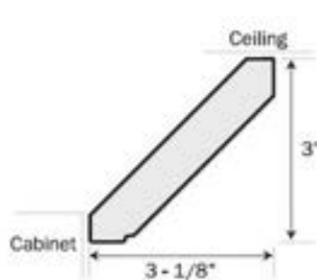
A140 Face Mount
