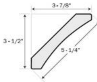
A170 Face Mount
