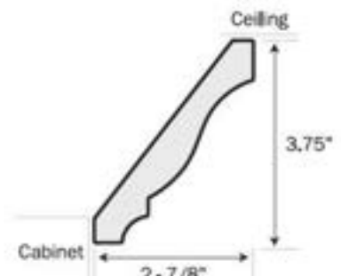
A141 Face Mount
